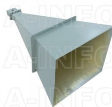
LB-650-20-C-NF Standard Gain Horn Antenna 1.12-1.7GHz 20dB Gain N Type Female
